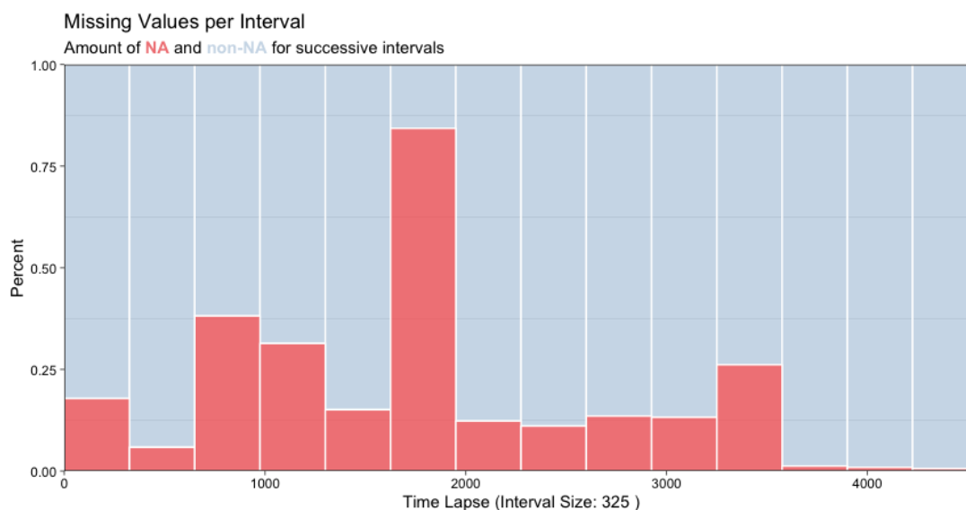
Figure 3: Example for ggplot_na_distribution2
